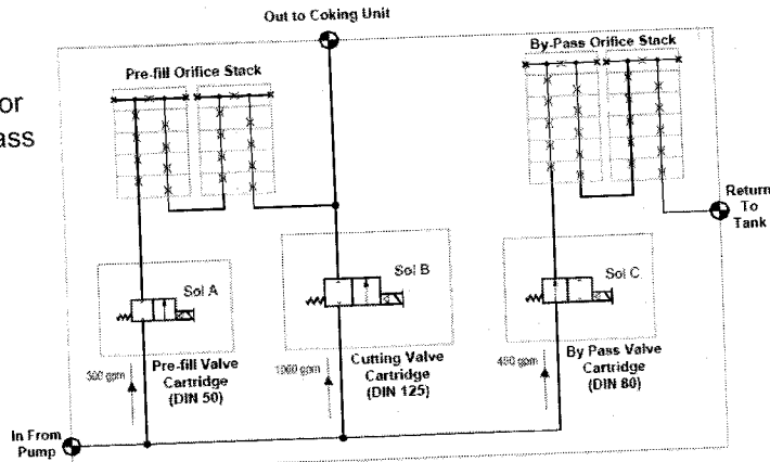
Typical Schematic Pump and Cutting Water Control
